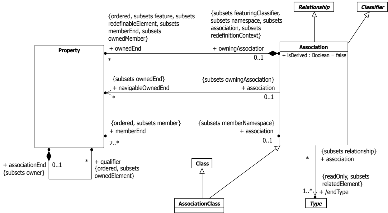
Figure 11.25 Associations
