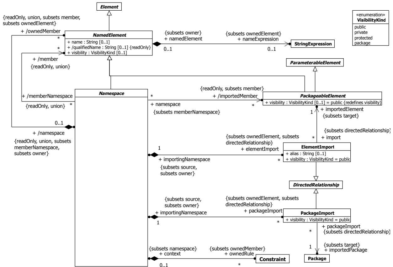
Figure 7.5 Namespaces
