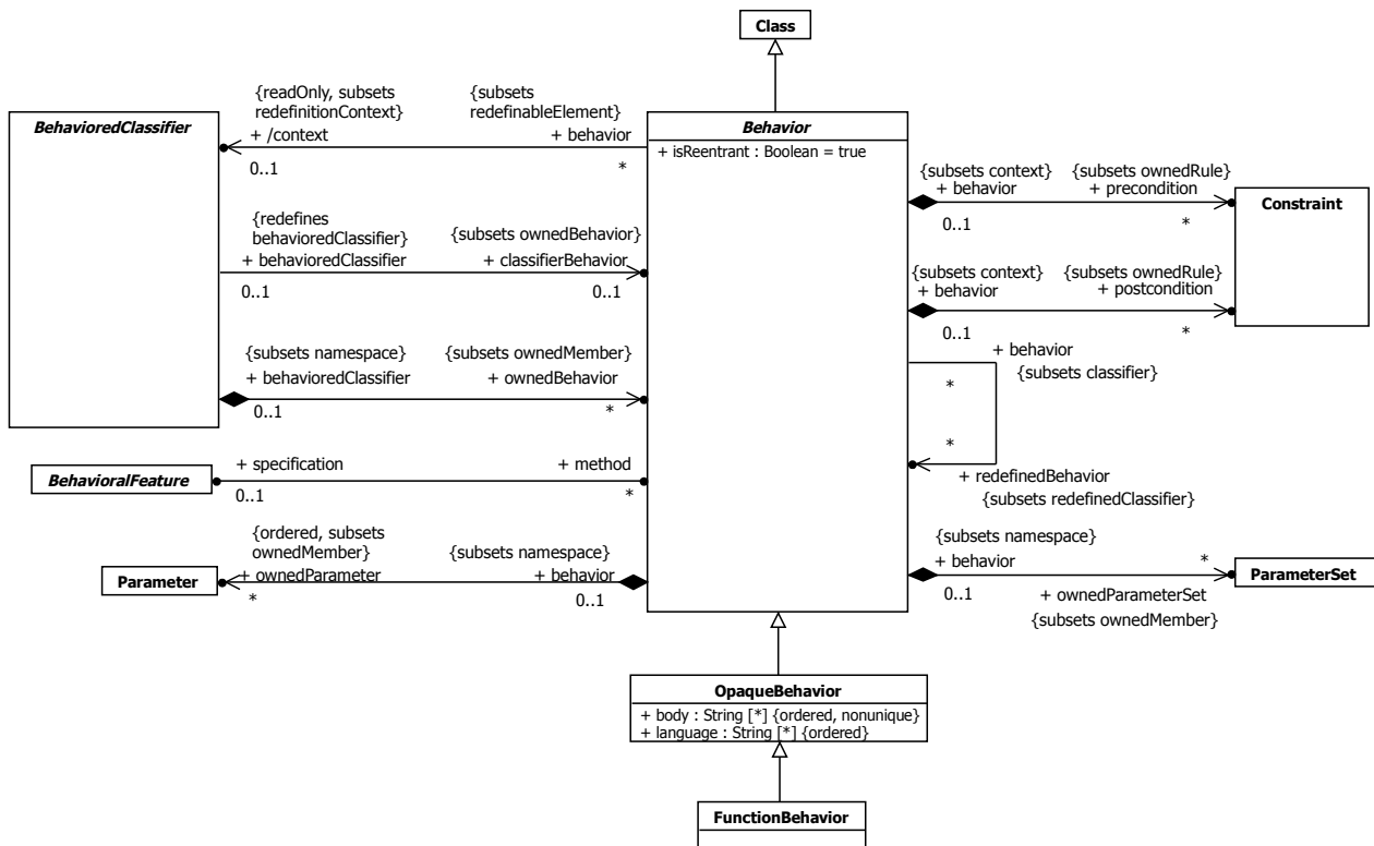
Figure 13.1 Behaviors
