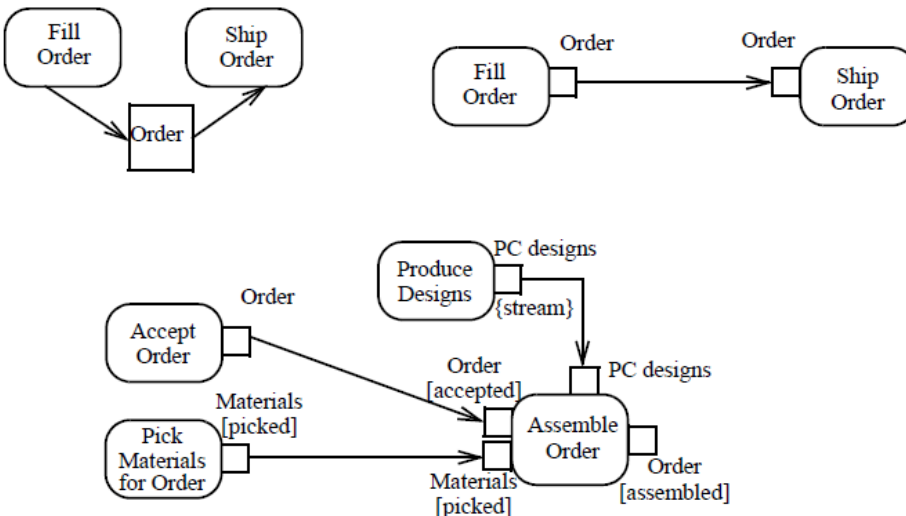
Figure 16.10 Pin examples
